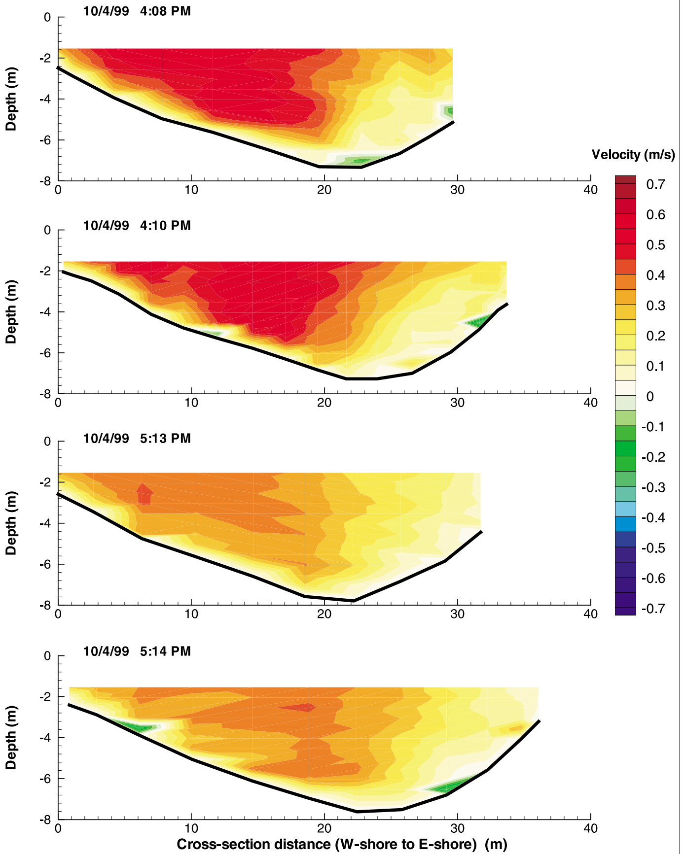
Figure G-174: Cross-Sectional Flow Distributions at GPA-20 on October 4, 1999
