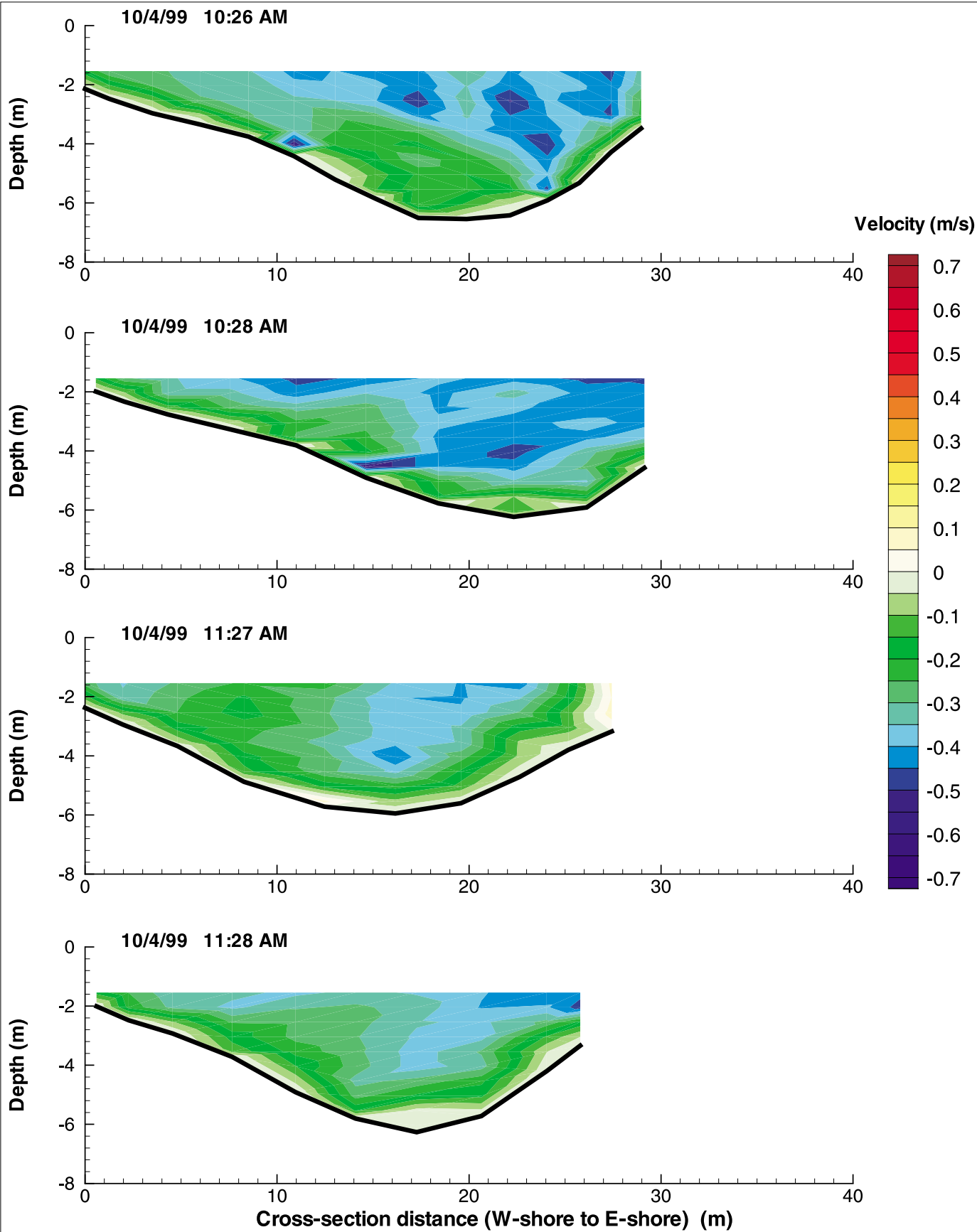
Figure G-172: Cross-Sectional Flow Distributions at GPA-20 on October 4, 1999
