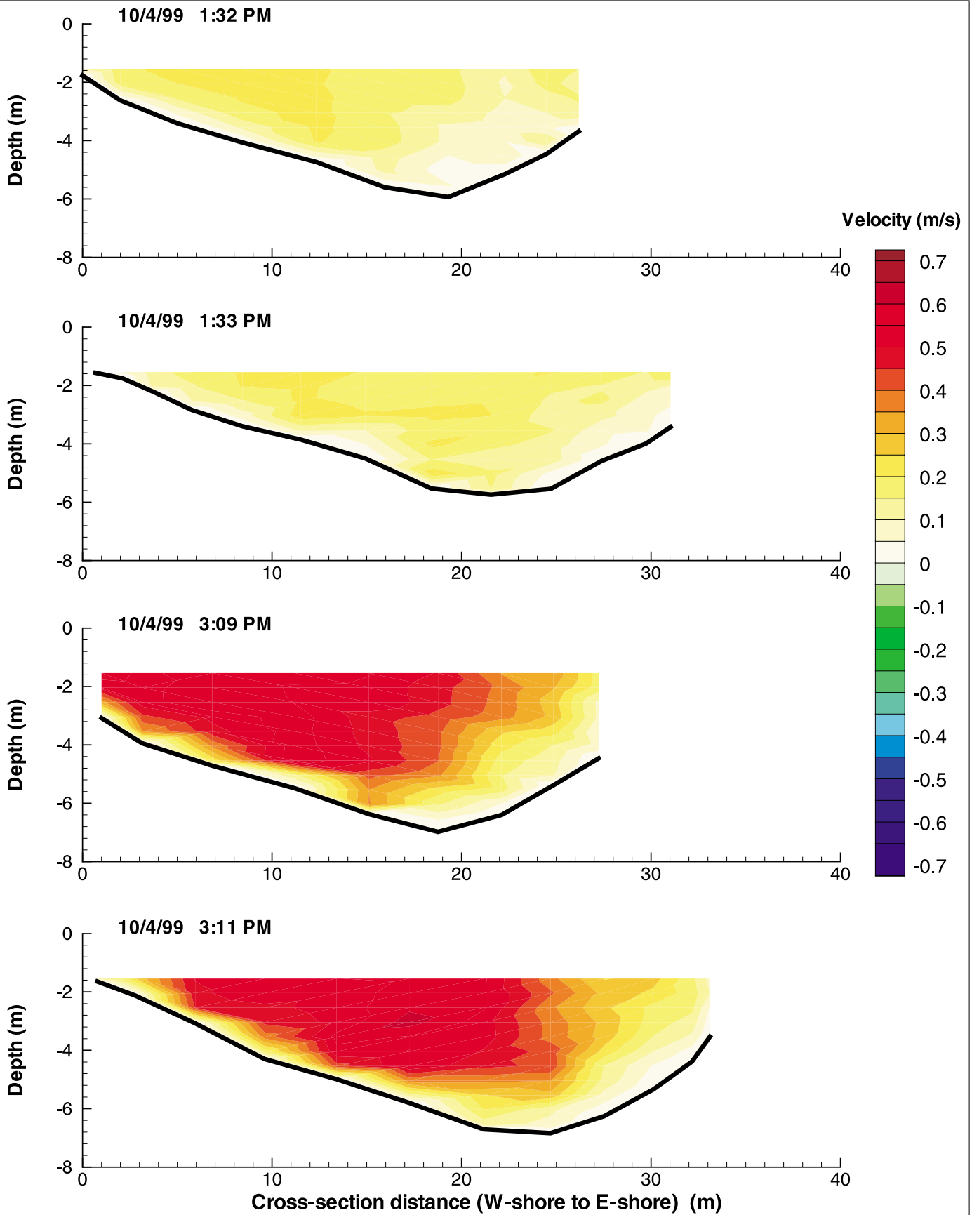
Figure G-173: Cross-Sectional Flow Distributions at GPA-20 on October 4, 1999
