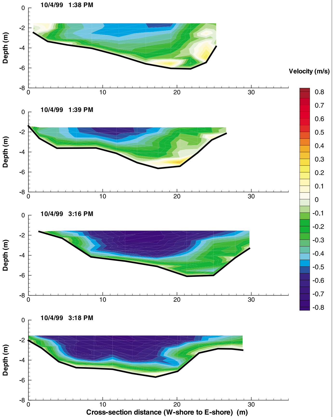
Figure G-170: Cross-Sectional Flow Distributions at GPA-19 on October 4, 1999
