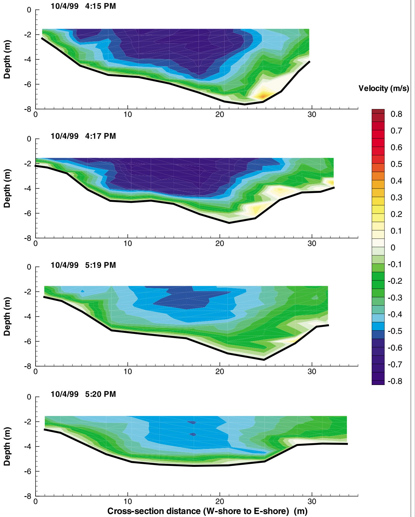
Figure G-171: Cross-Sectional Flow Distributions at GPA-19 on October 4, 1999
