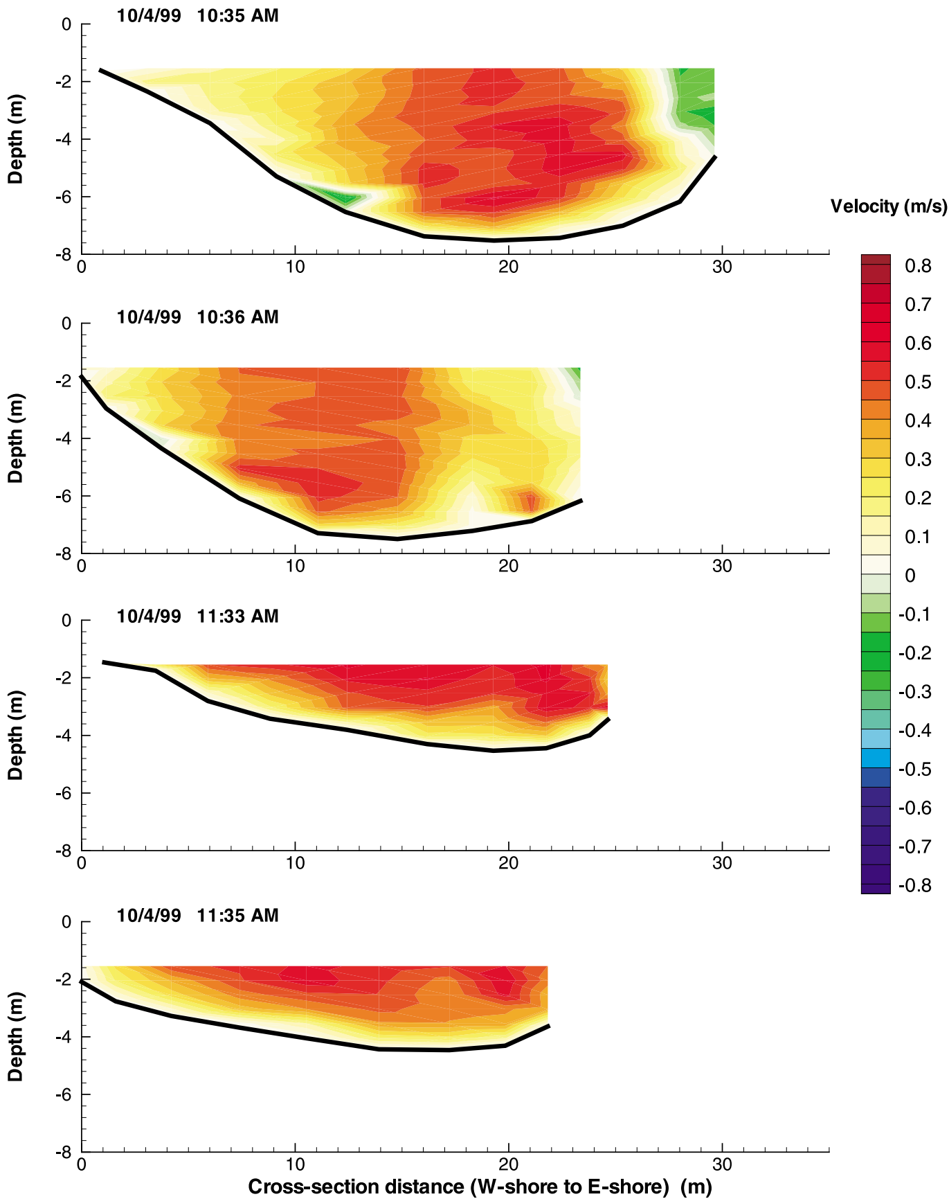
Figure G-169: Cross-Sectional Flow Distributions at GPA-19 on October 4, 1999
