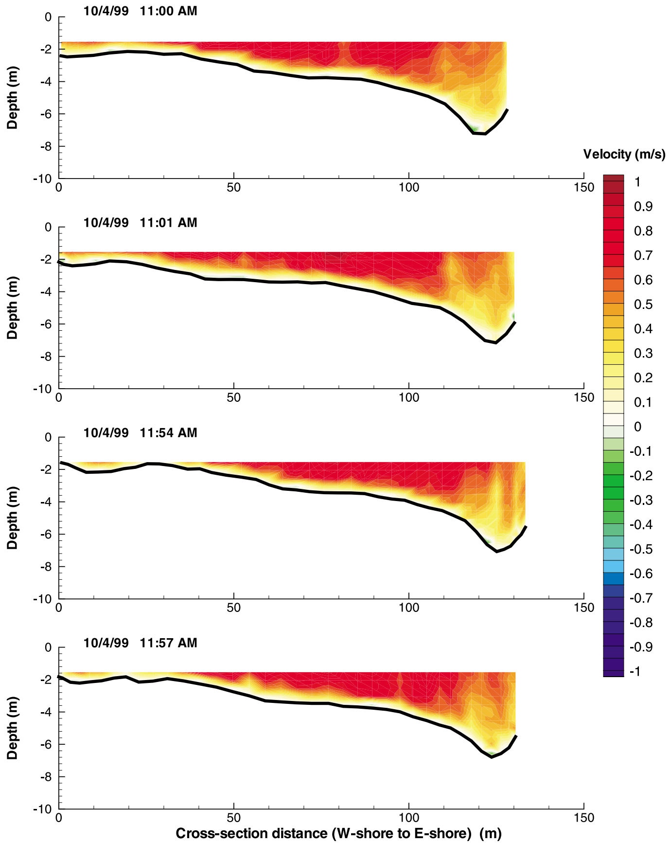
Figure G-166: Cross-Sectional Flow Distributions at GPA-18 on October 4, 1999
