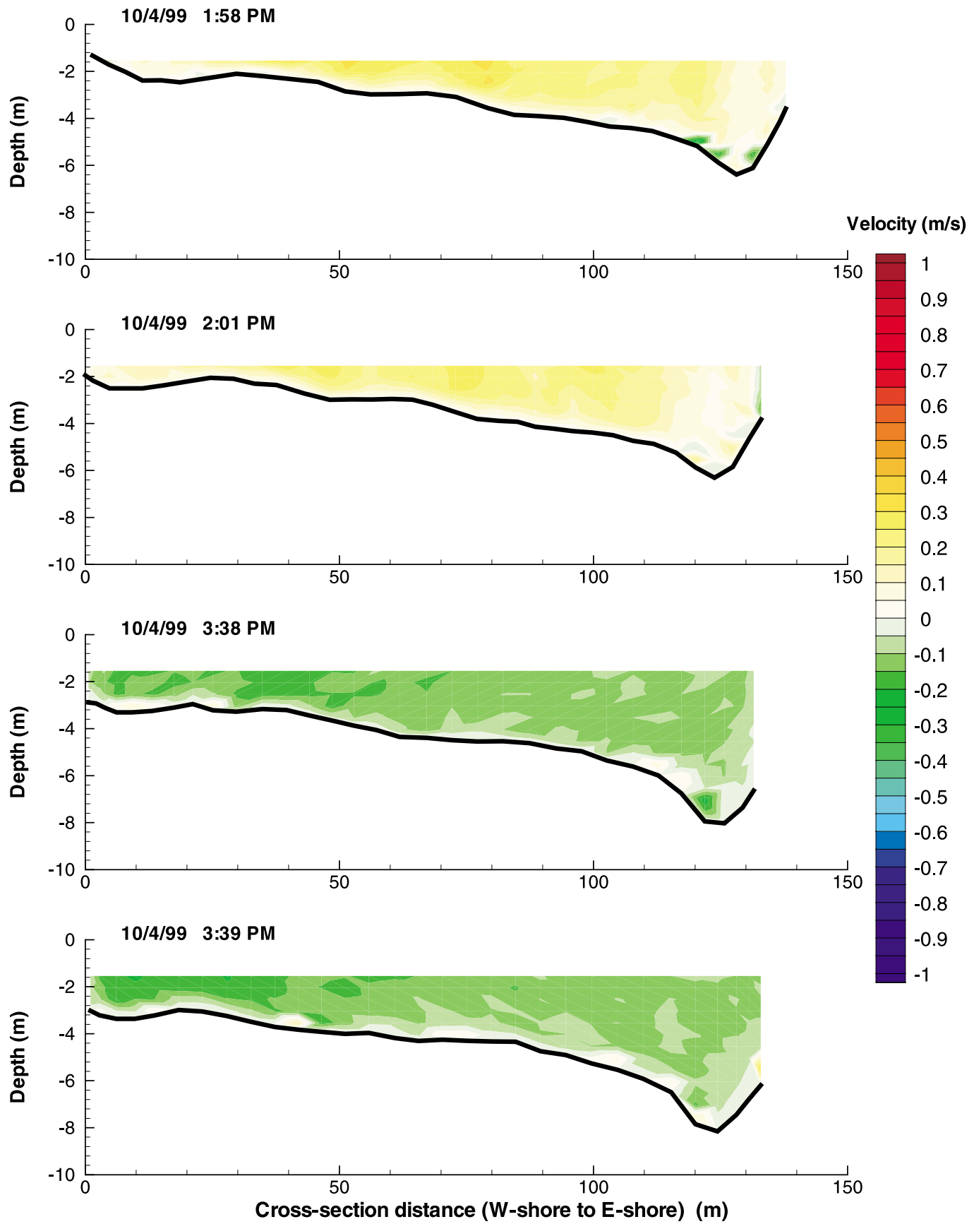
Figure G-167: Cross-Sectional Flow Distributions at GPA-18 on October 4, 1999
