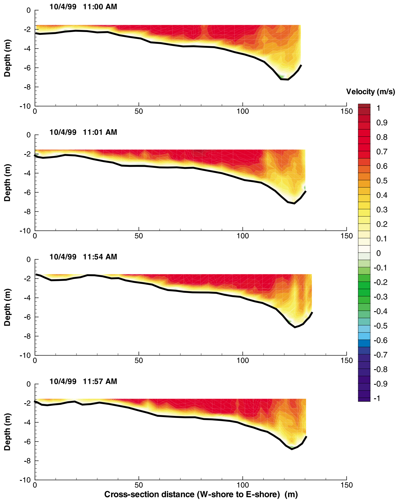
Figure G-163: Cross-Sectional Flow Distributions at GPA-16 on October 4, 1999
