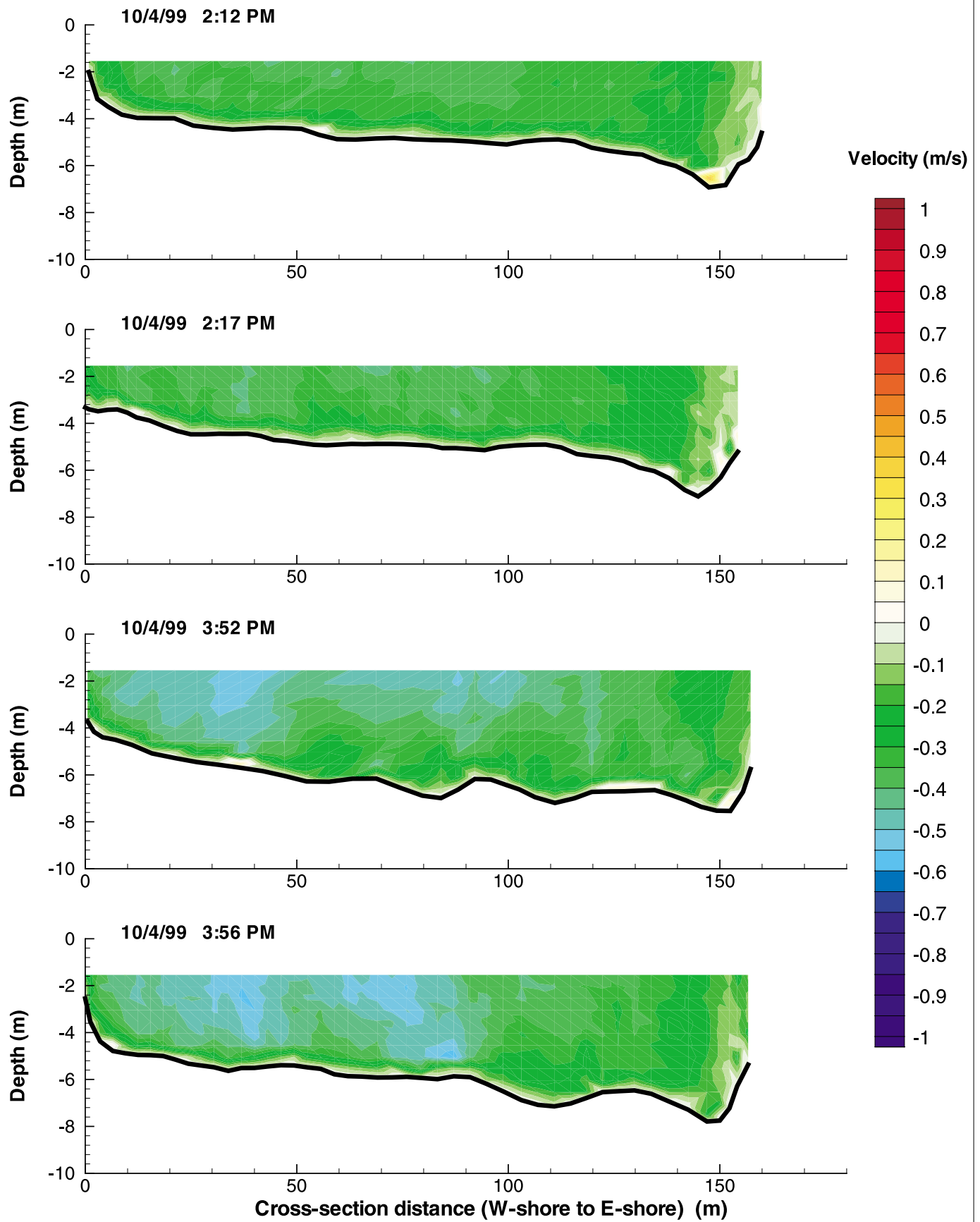
Figure G-161: Cross-Sectional Flow Distributions at GPA-14 on October 4, 1999
