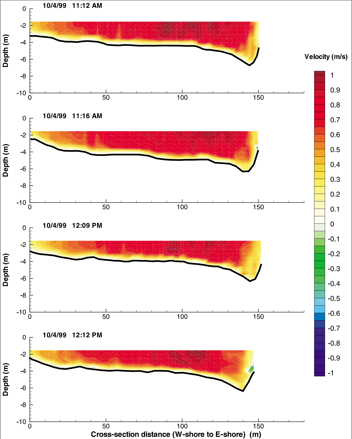
Figure G-160: Cross-Sectional Flow Distributions at GPA-14 on October 4, 1999
