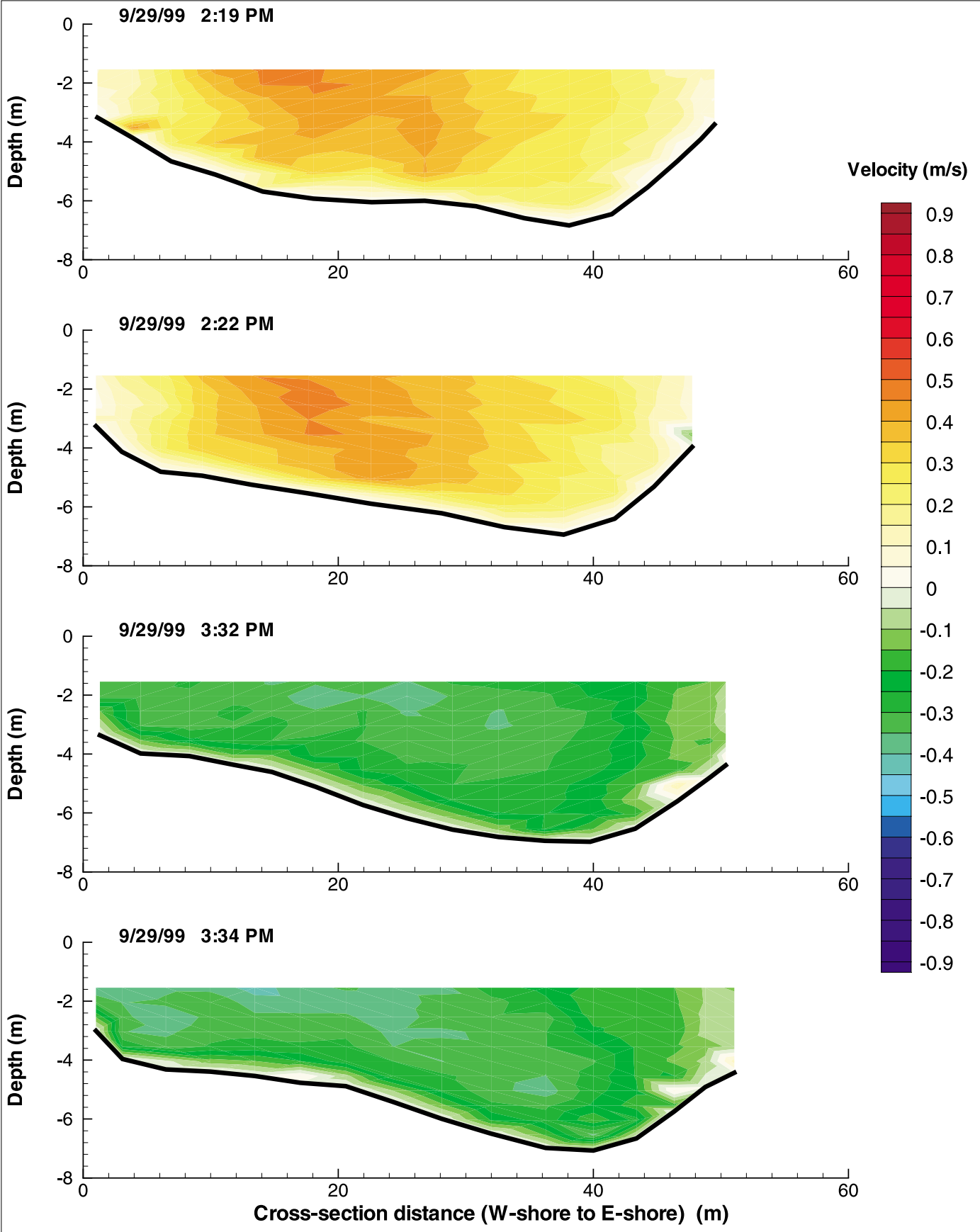
Figure G-148: Cross-Sectional Flow Distributions at MC on September 29, 1999
