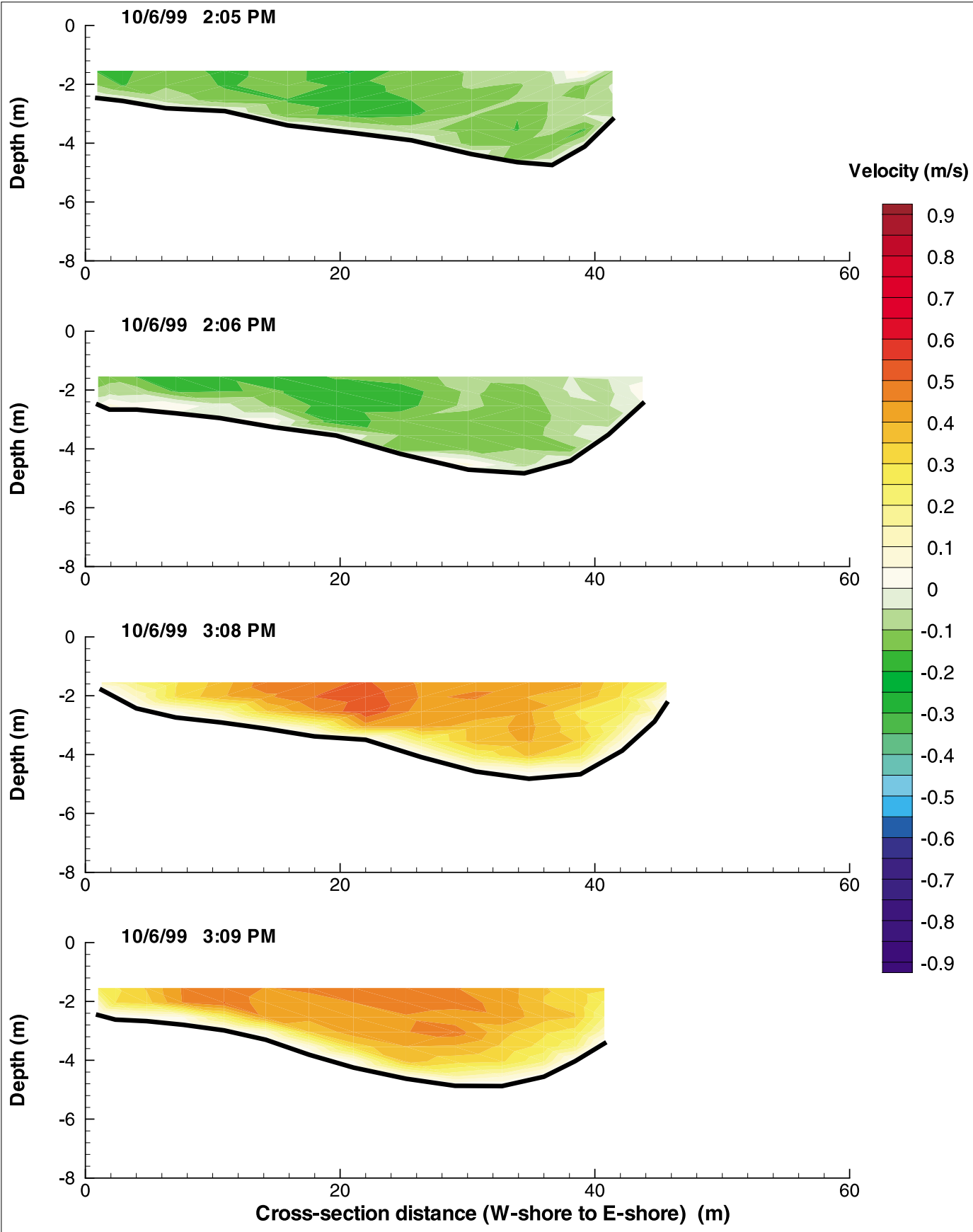
Figure G-151: Cross-Sectional Flow Distributions at MC on October 6, 1999
