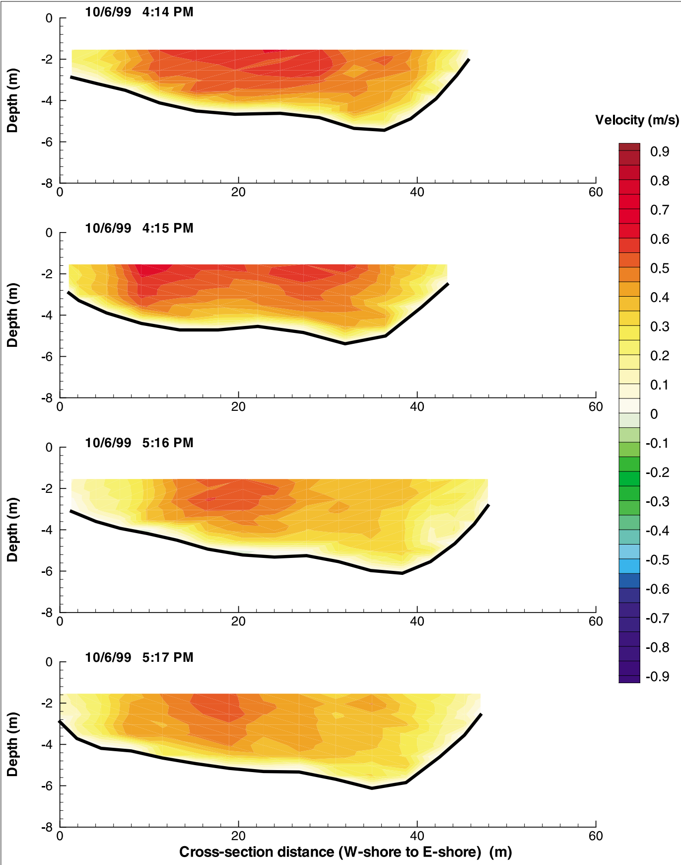
Figure G-152: Cross-Sectional Flow Distributions at MC on October 6, 1999
