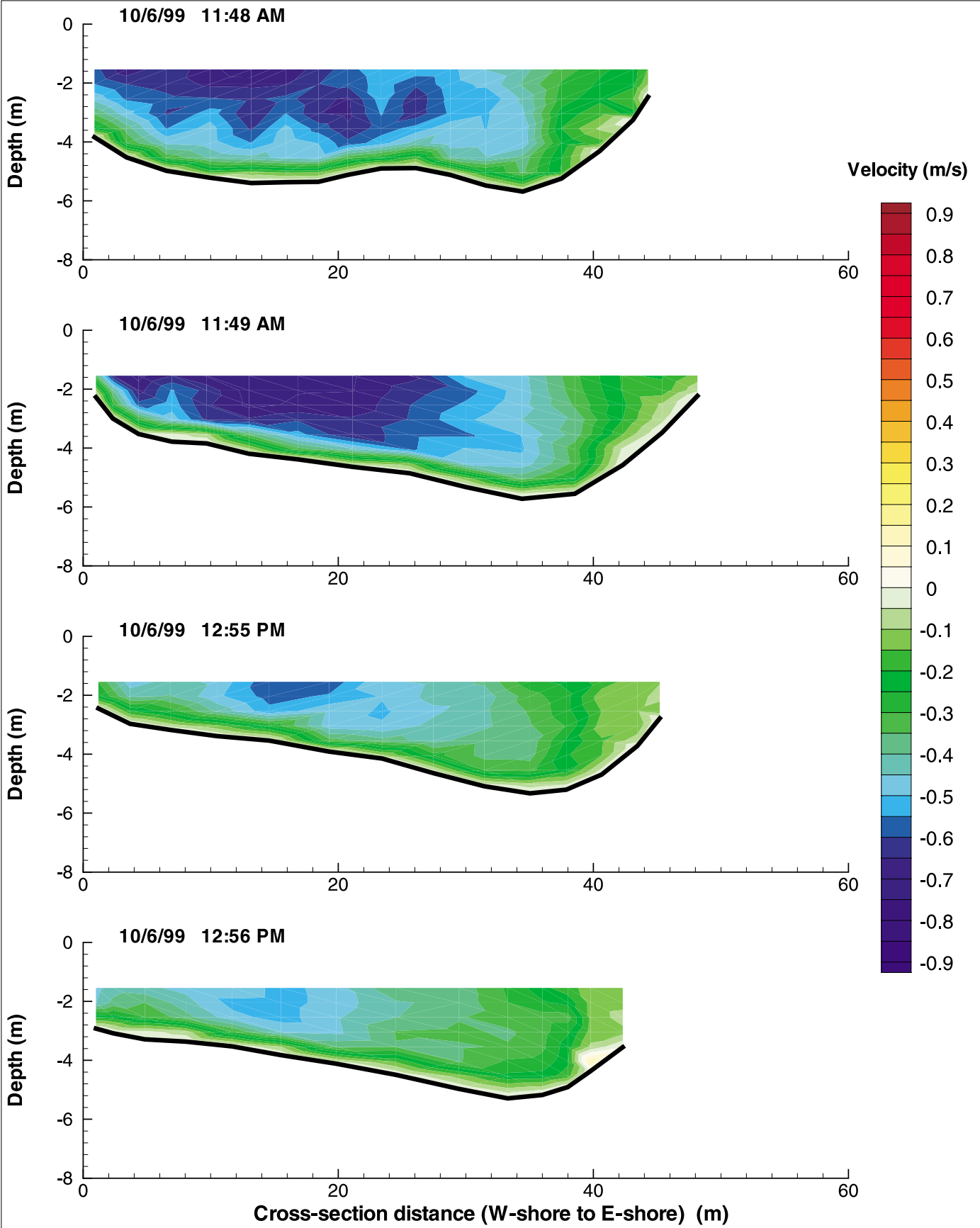
Figure G-150: Cross-Sectional Flow Distributions at MC on October 6, 1999
