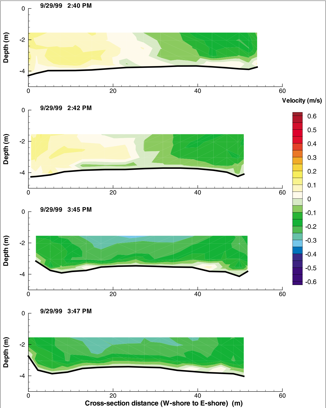
Figure G-136: Cross-Sectional Flow Distributions at LBR1 on September 29, 1999
