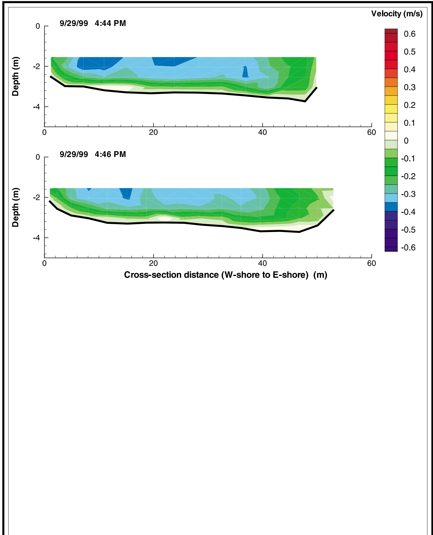
Figure G-137: Cross-Sectional Flow Distributions at LBR1 on September 29, 1999
