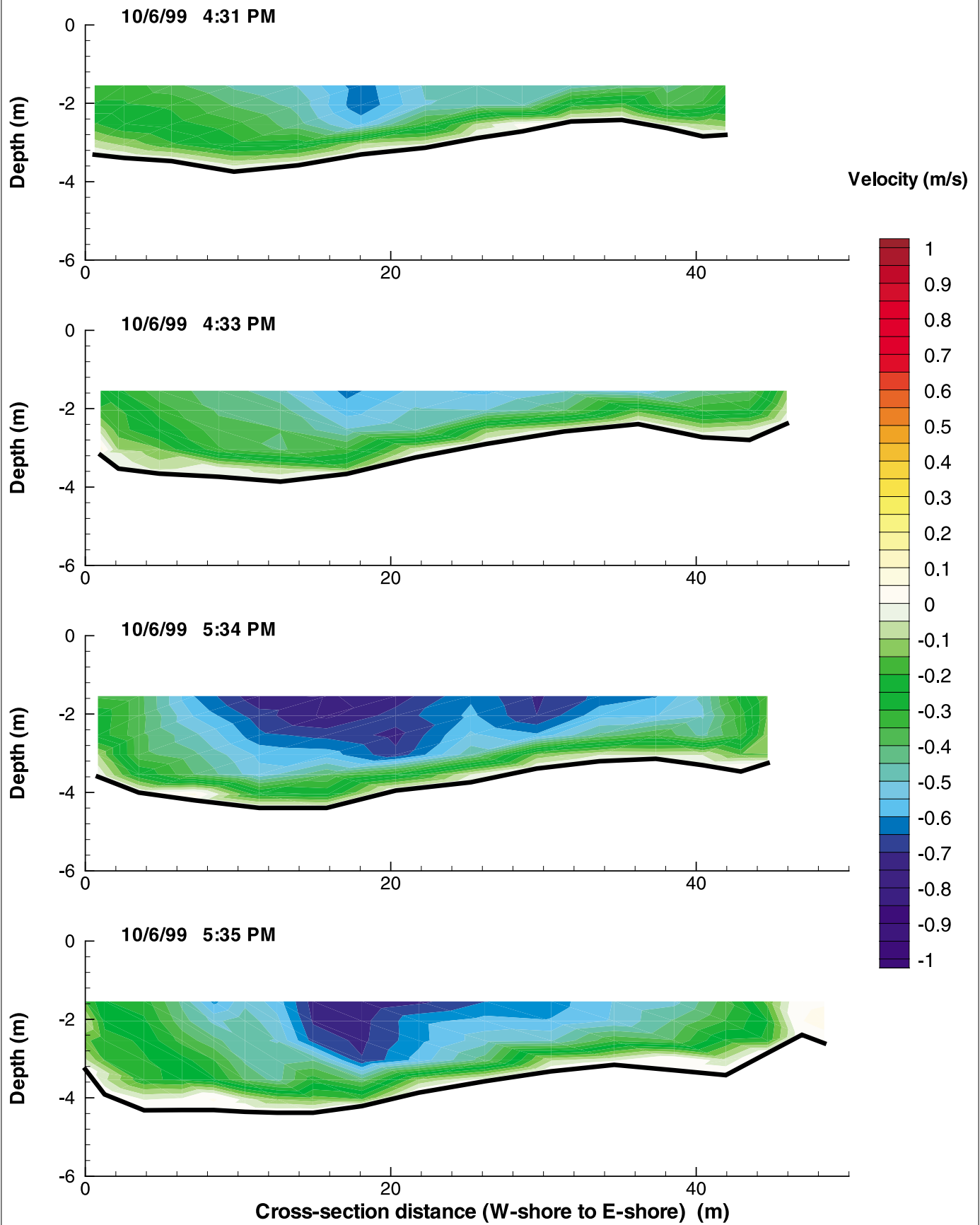
Figure G-135: Cross-Sectional Flow Distributions at MR1 on October 6, 1999
