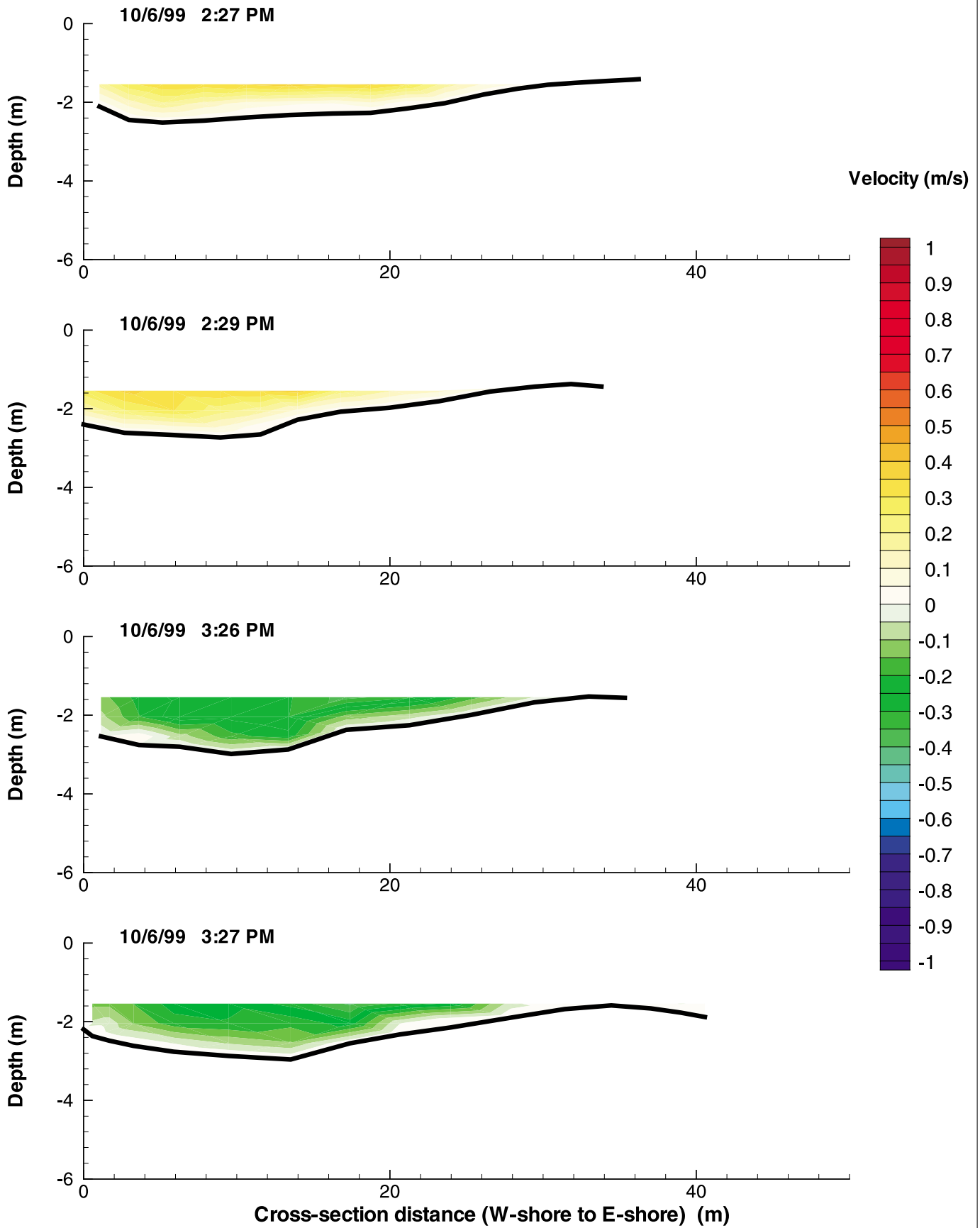
Figure G-134: Cross-Sectional Flow Distributions at MR1 on October 6, 1999
