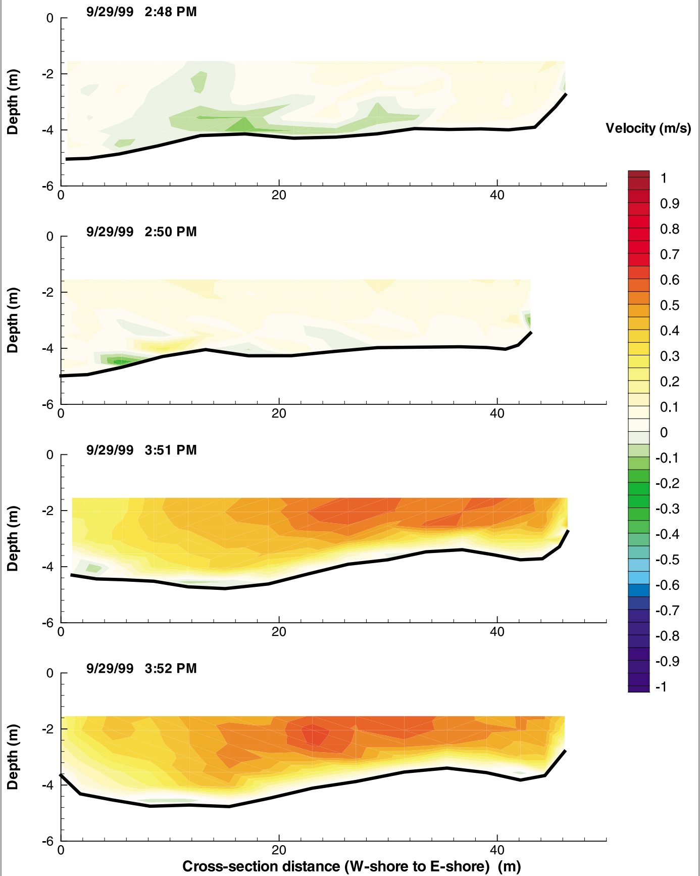
Figure G-131: Cross-Sectional Flow Distributions at MR1 on September 29, 1999
