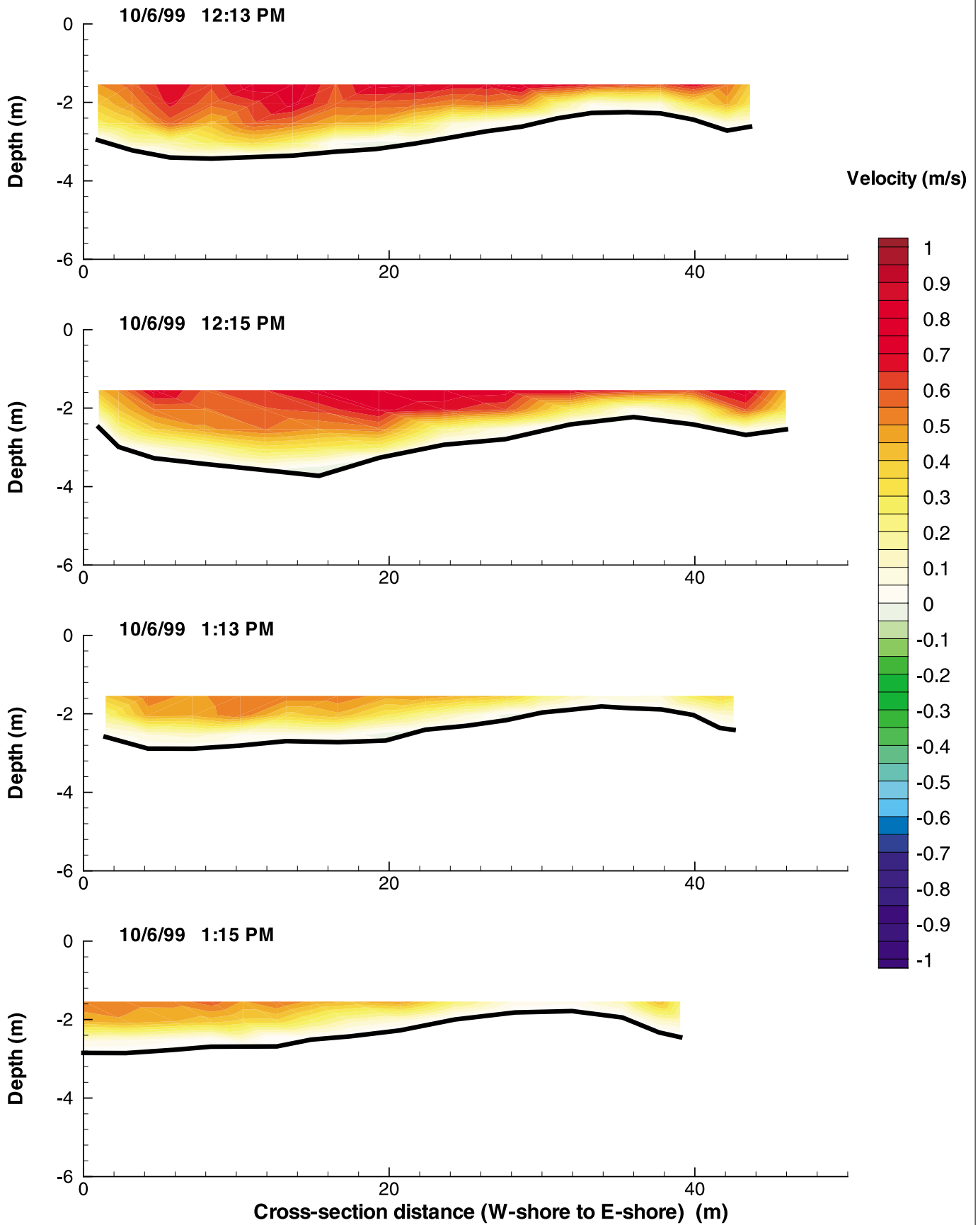
Figure G-133: Cross-Sectional Flow Distributions at MR1 on October 6, 1999
