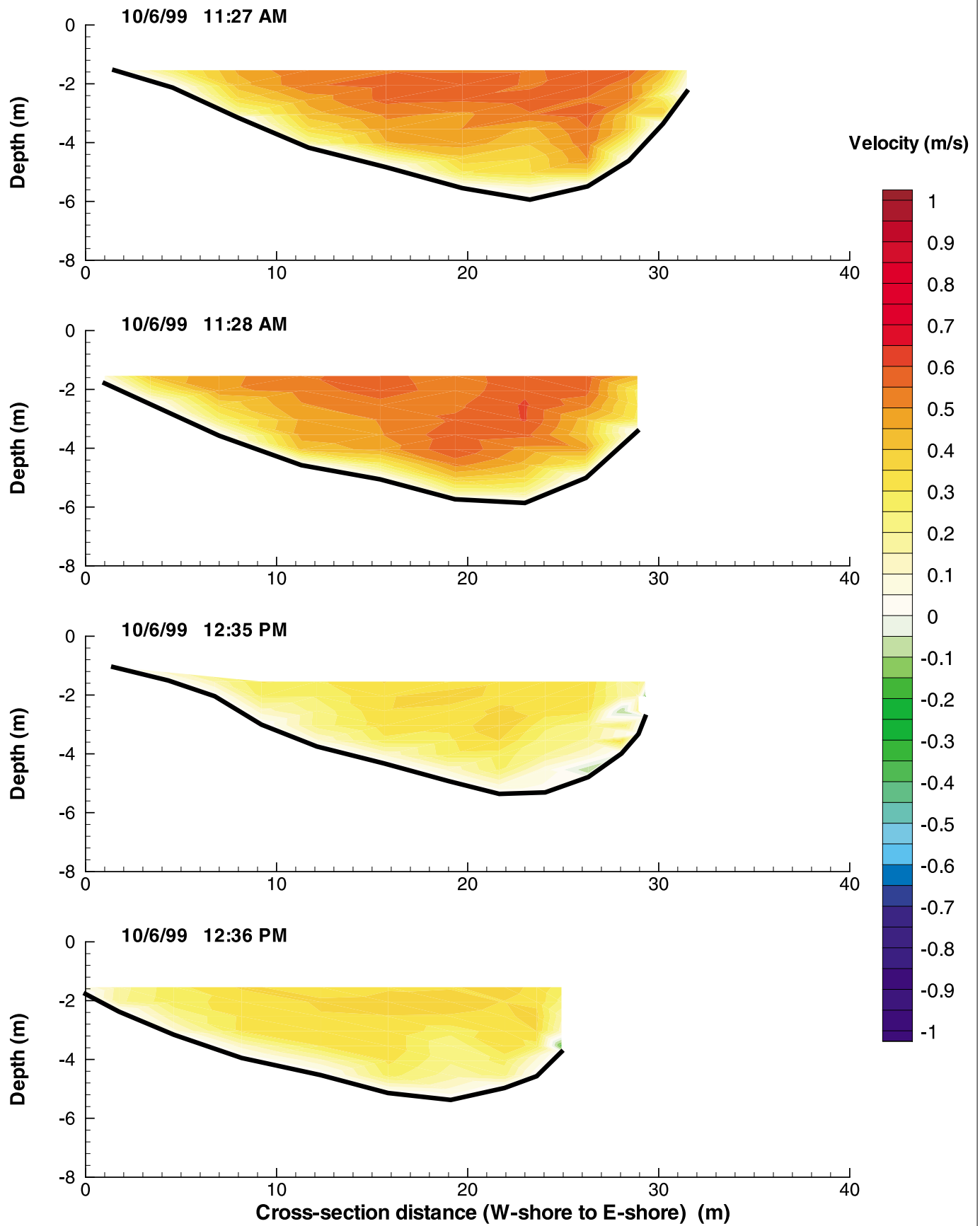
Figure G-120: Cross-Sectional Flow Distributions at KC on October 6, 1999
