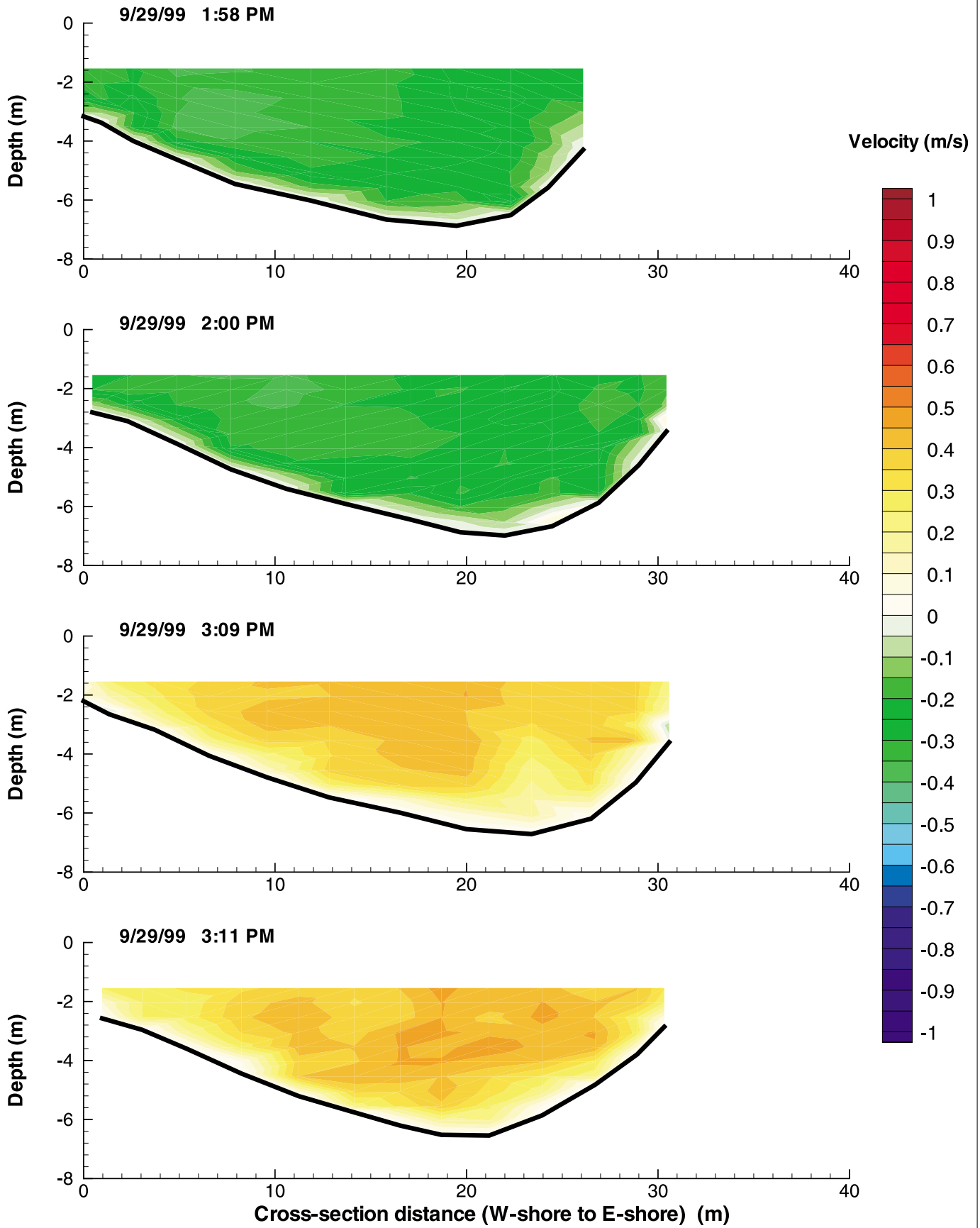
Figure G-118: Cross-Sectional Flow Distributions at KC on September 29, 1999
