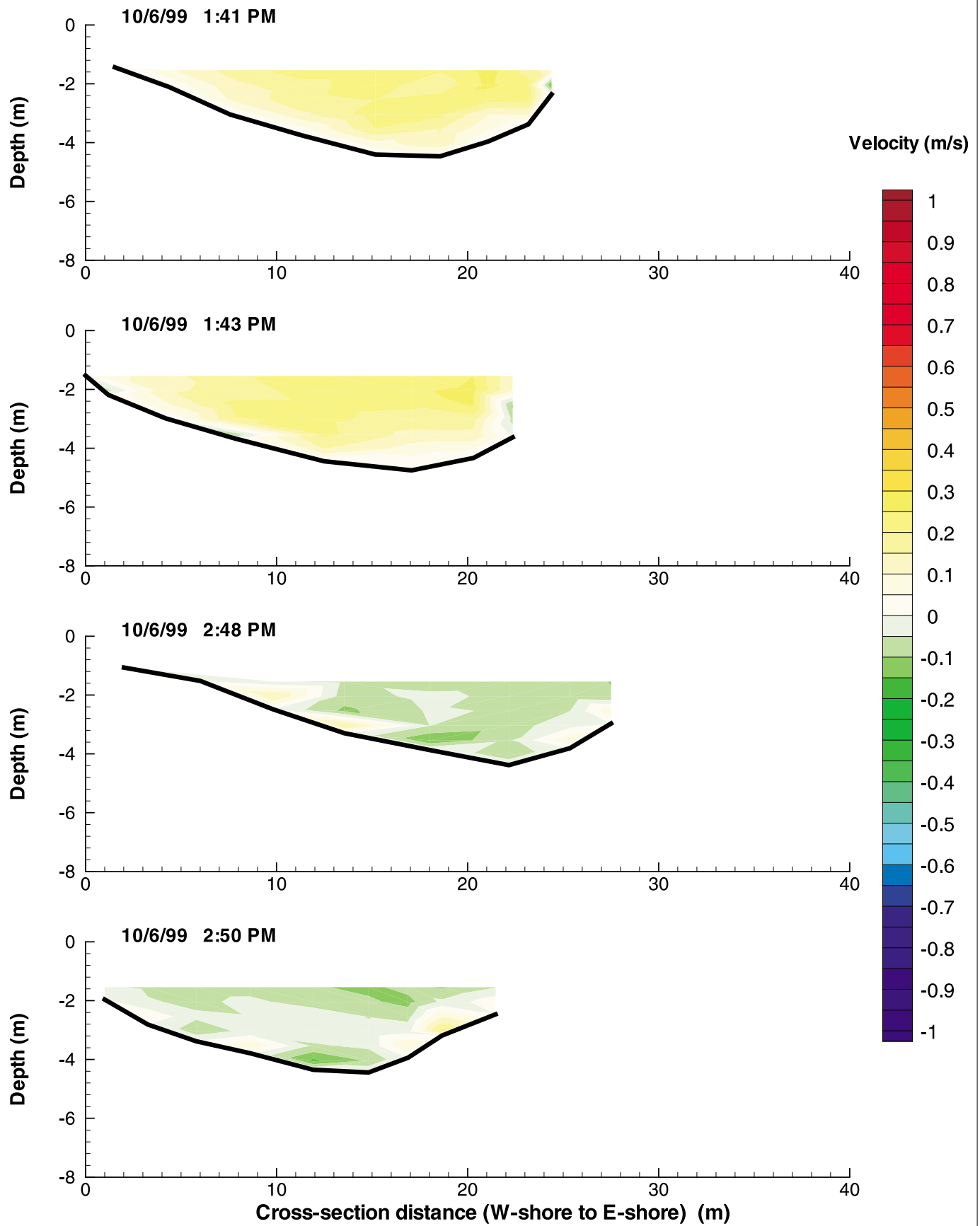
Figure G-121: Cross-Sectional Flow Distributions at KC on October 6, 1999
