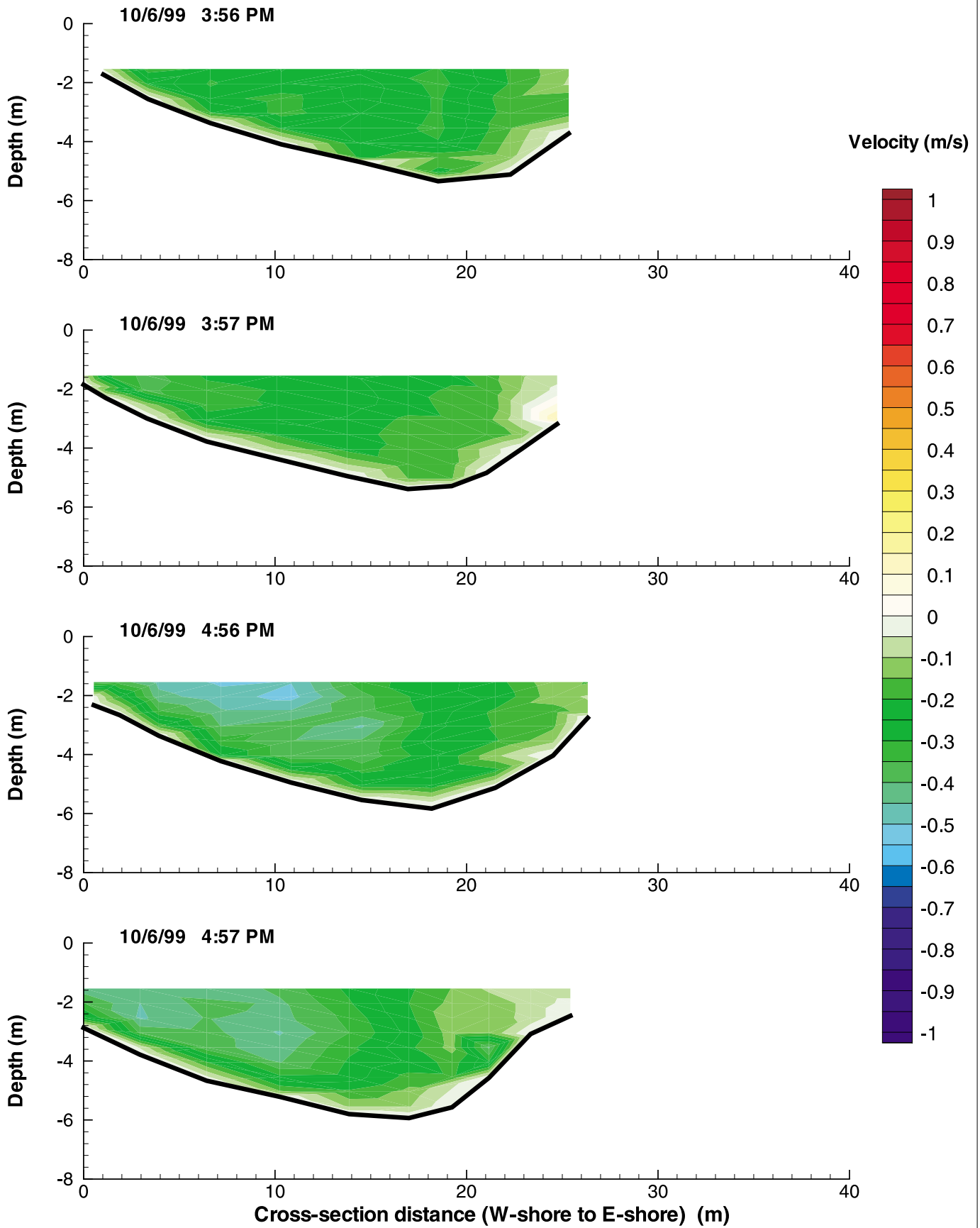
Figure G-122: Cross-Sectional Flow Distributions at KC on October 6, 1999
