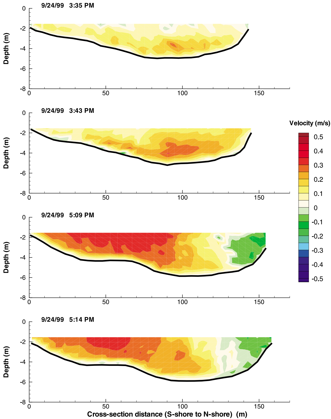
Figure G-117: Cross-Sectional Flow Distributions at WR on September 24, 1999
