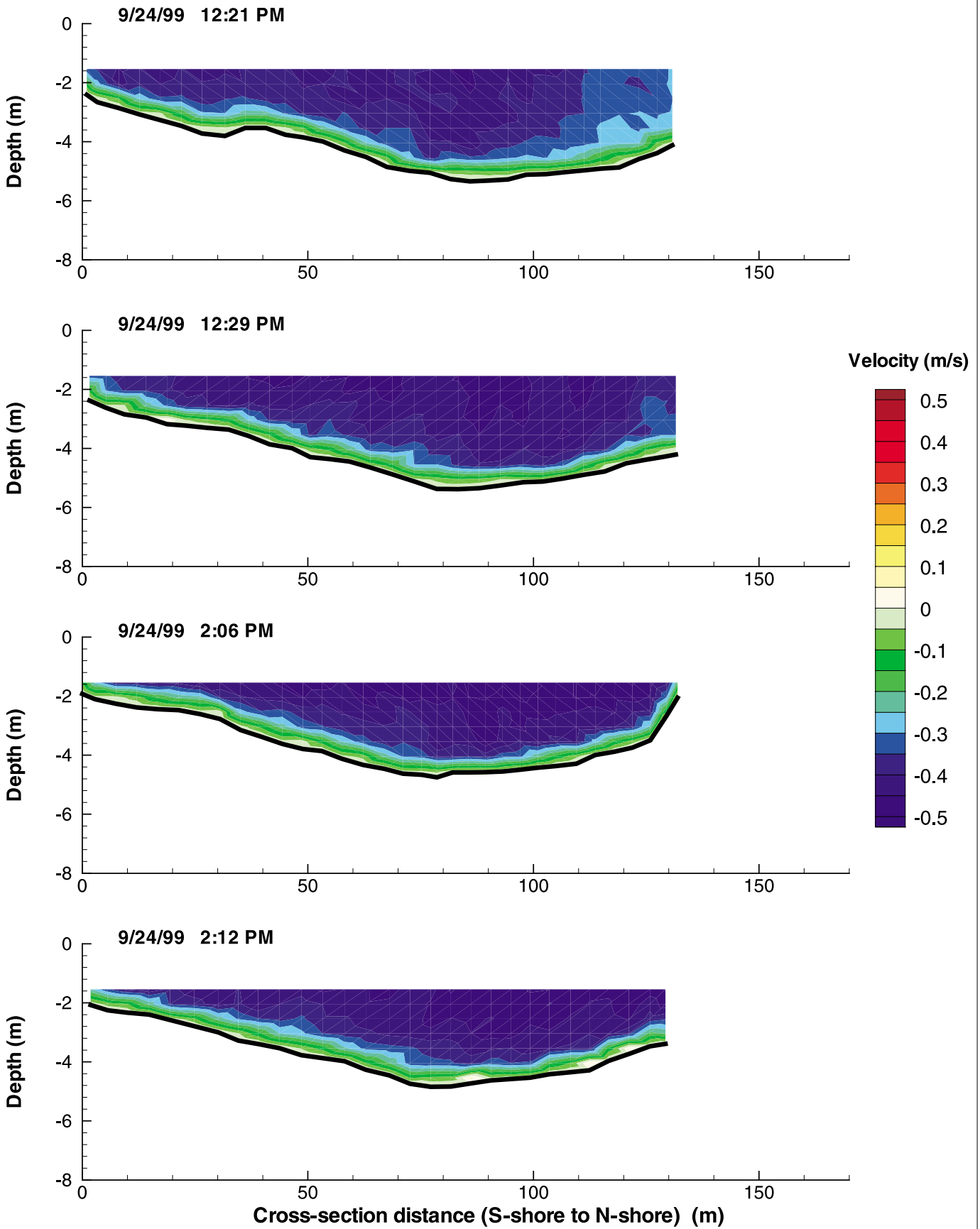
Figure G-116: Cross-Sectional Flow Distributions at WR on September 24, 1999
