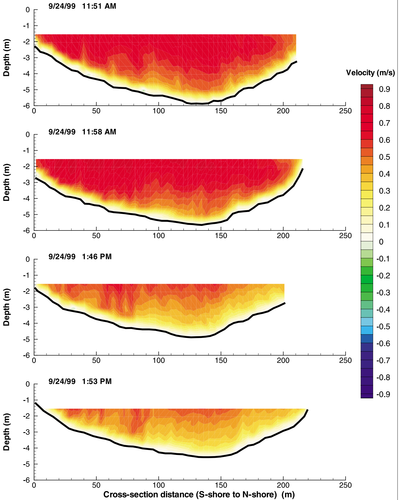
Figure G-114: Cross-Sectional Flow Distributions at SCU on September 24, 1999
