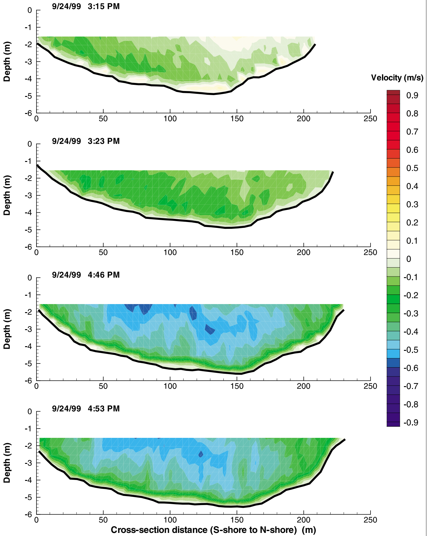
Figure G-115: Cross-Sectional Flow Distributions at SCU on September 24, 1999
