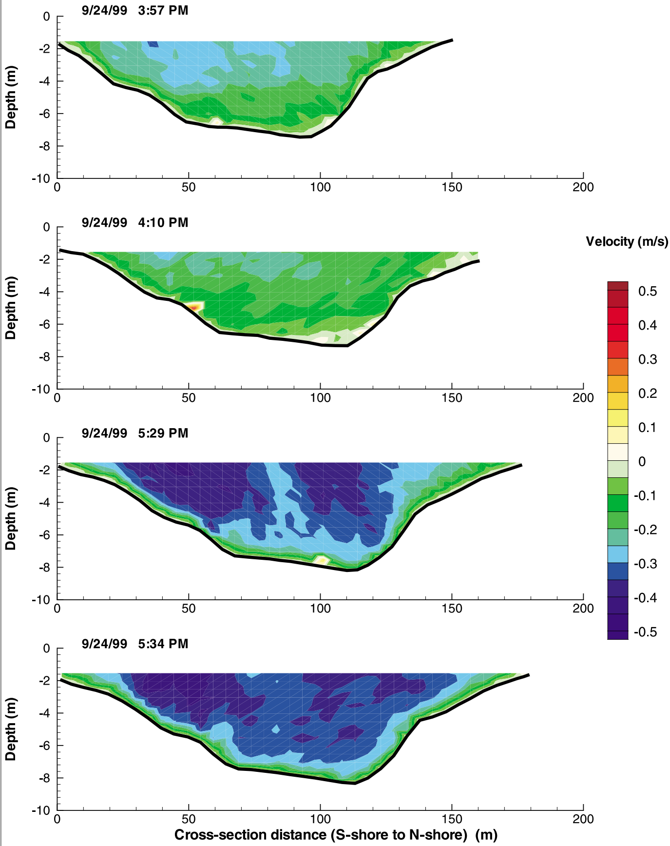
Figure G-113: Cross-Sectional Flow Distributions at EIW on September 24, 1999
