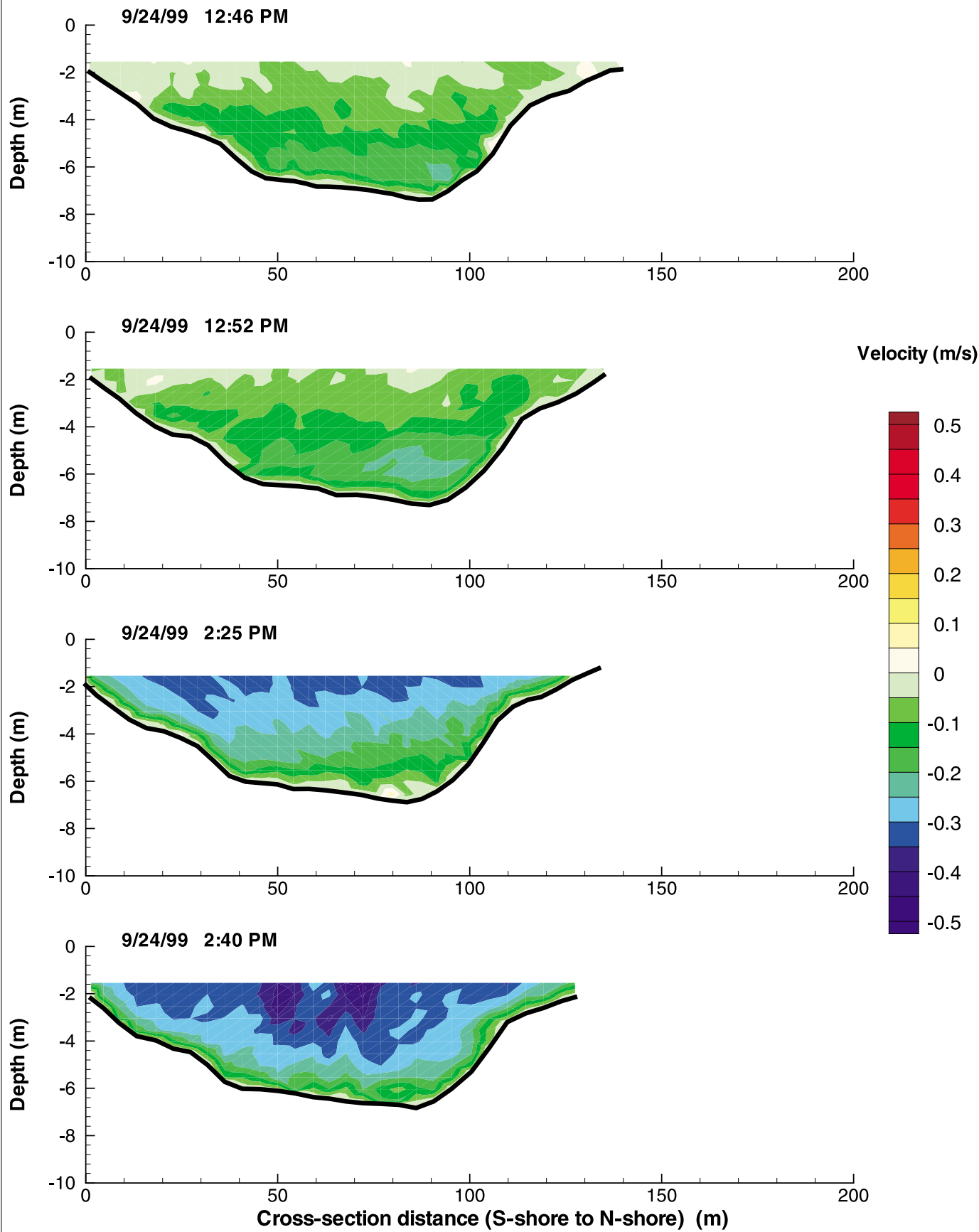
Figure G-112: Cross-Sectional Flow Distributions at EIW on September 24, 1999
