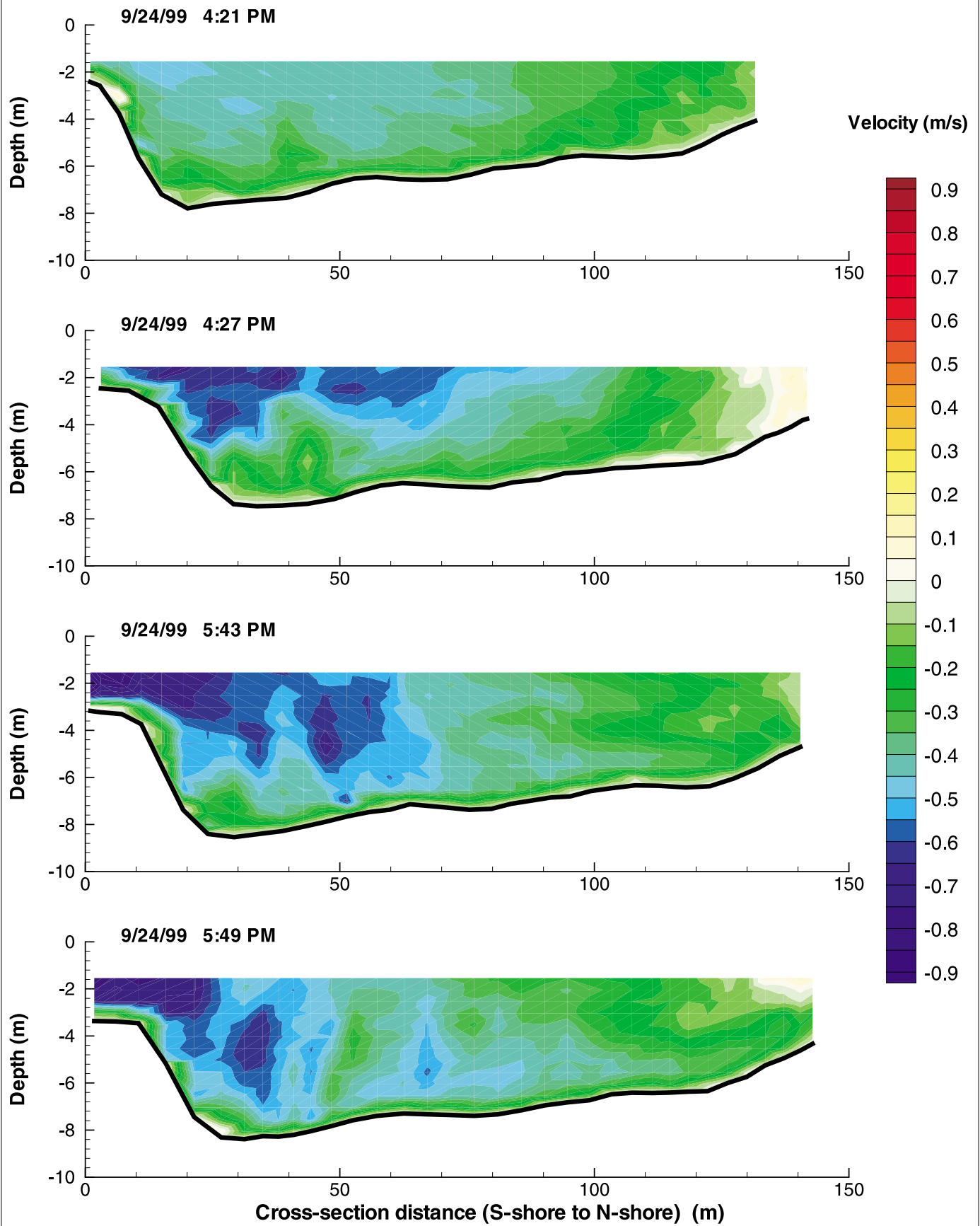
Figure G-111: Cross-Sectional Flow Distributions at EIE on September 24, 1999
