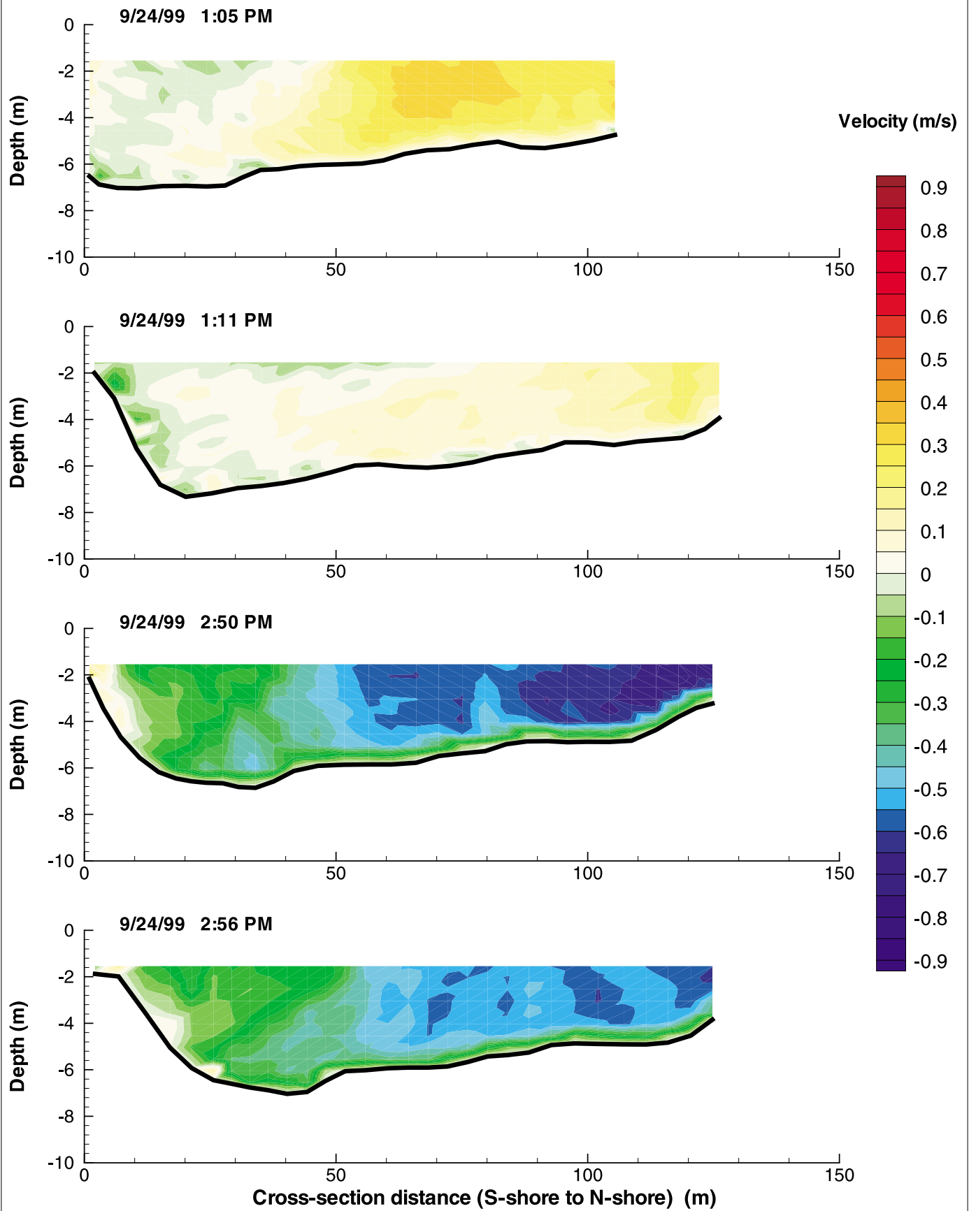
Figure G-110: Cross-Sectional Flow Distributions at EIE on September 24, 1999
