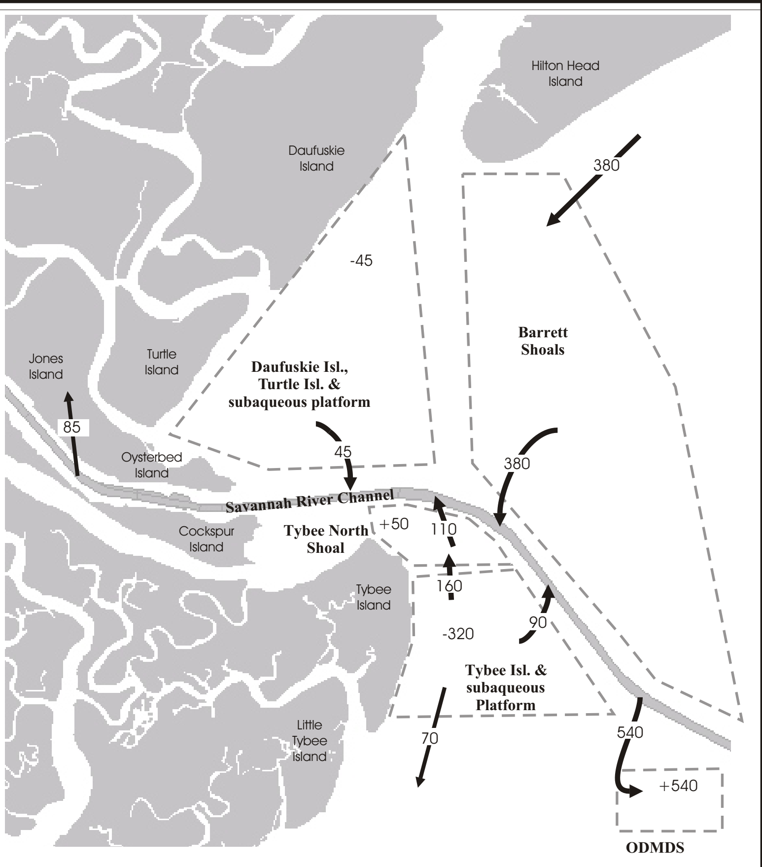
Figure 8-29 Final sediment budget
