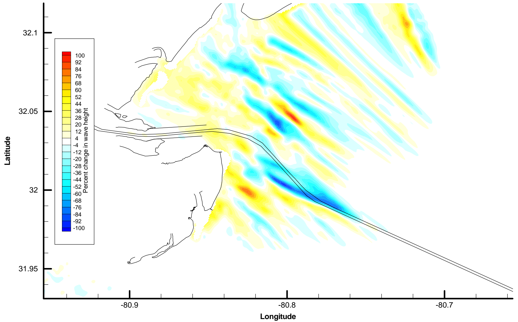
Figure 7-29 Simulated change in Case 5 wave conditions from 1854 to present
