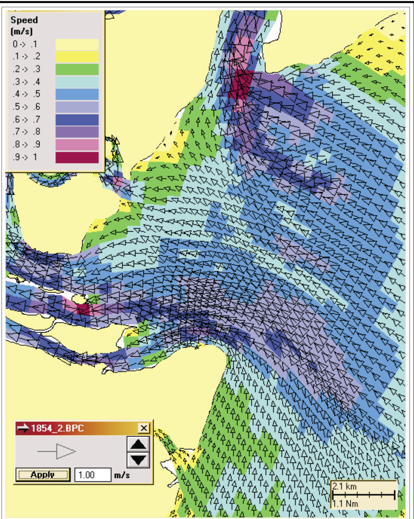
Figure 6-19 Simulated peak flood currents for average tidal range (1854 conditions). Current velocity shown as vectors, and current speed shown as color contours.
