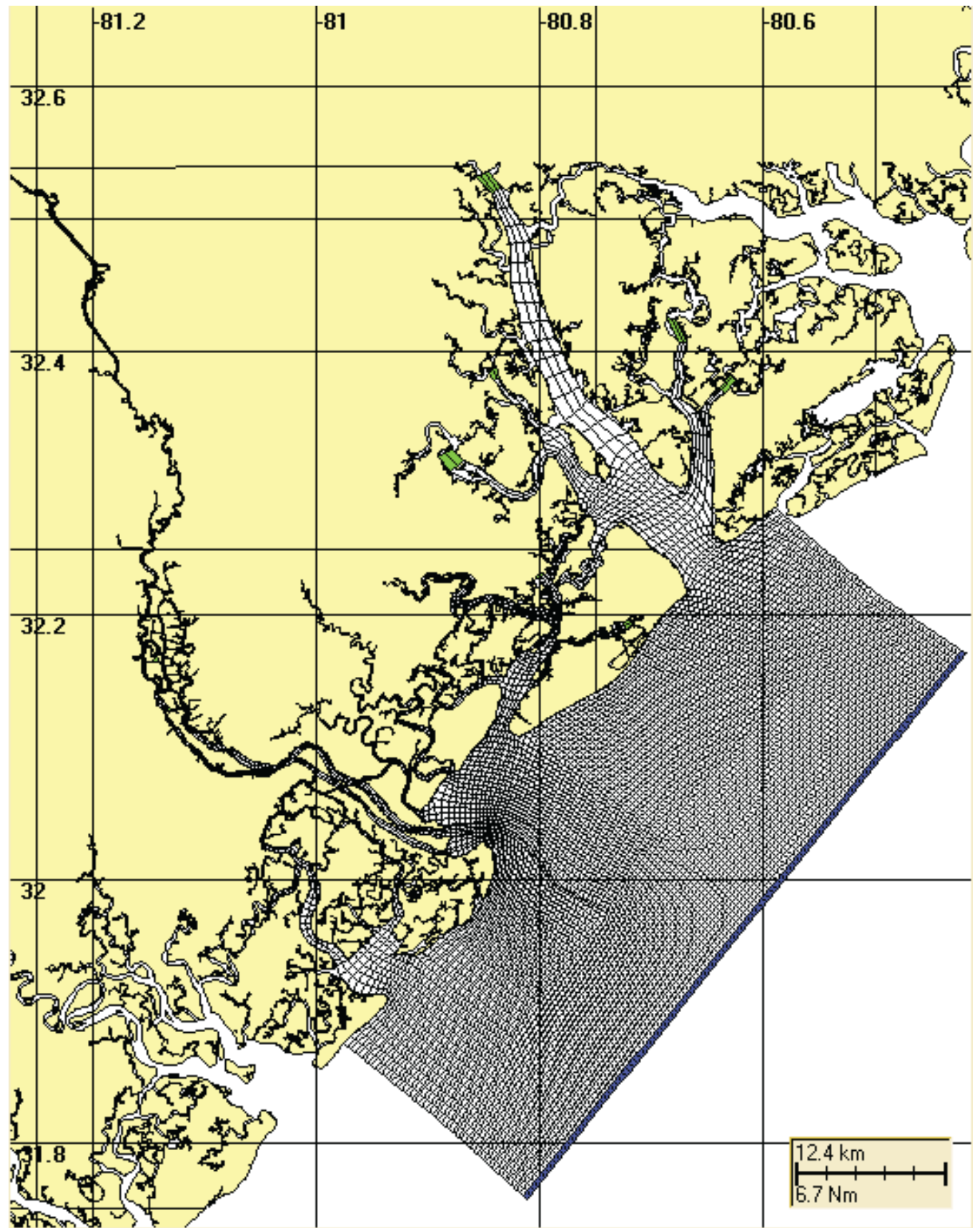
Figure 6-1 Hydrodynamic model grid
