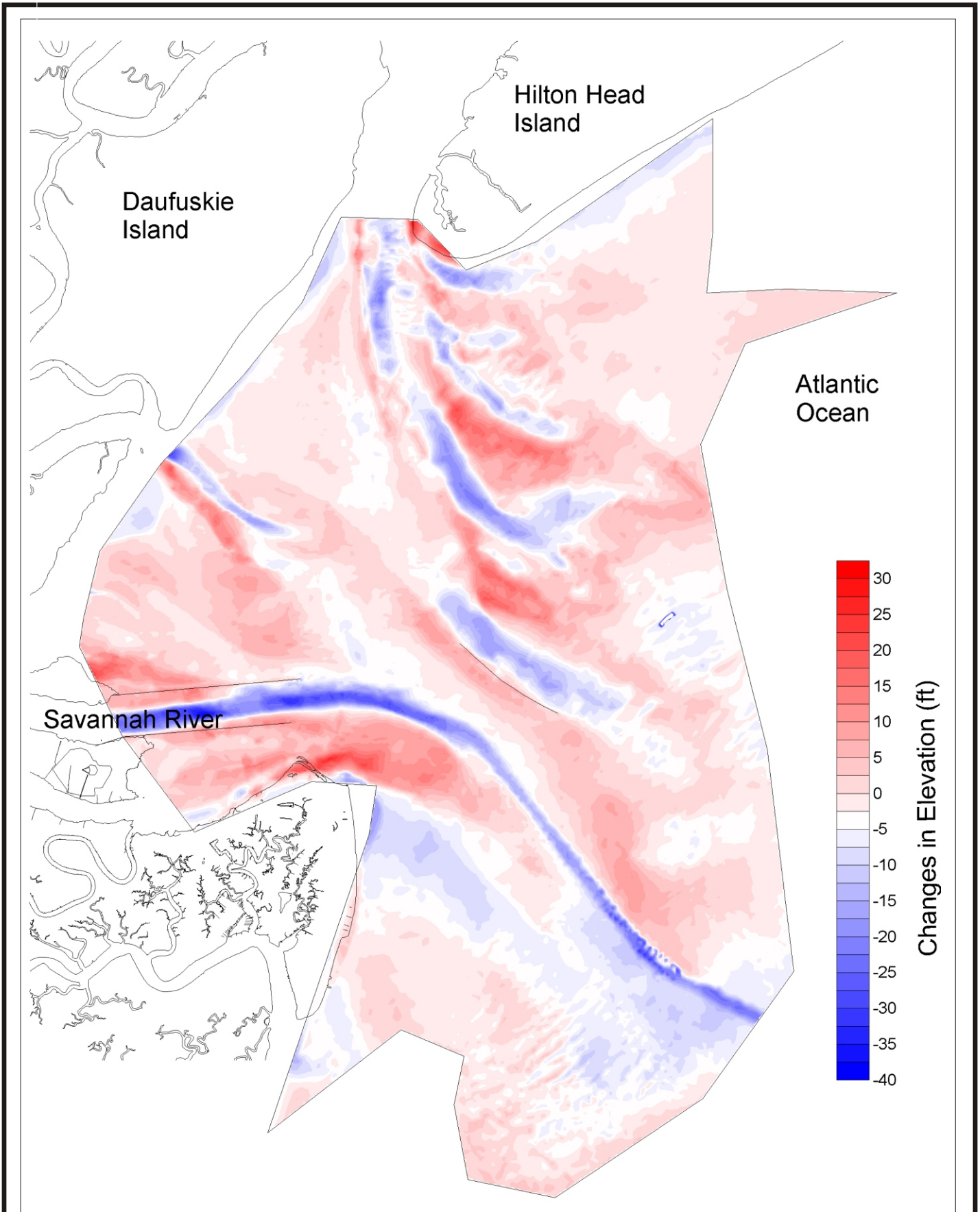
Figure 4-19 1854 to 1970/1980 Changes in Elevation
