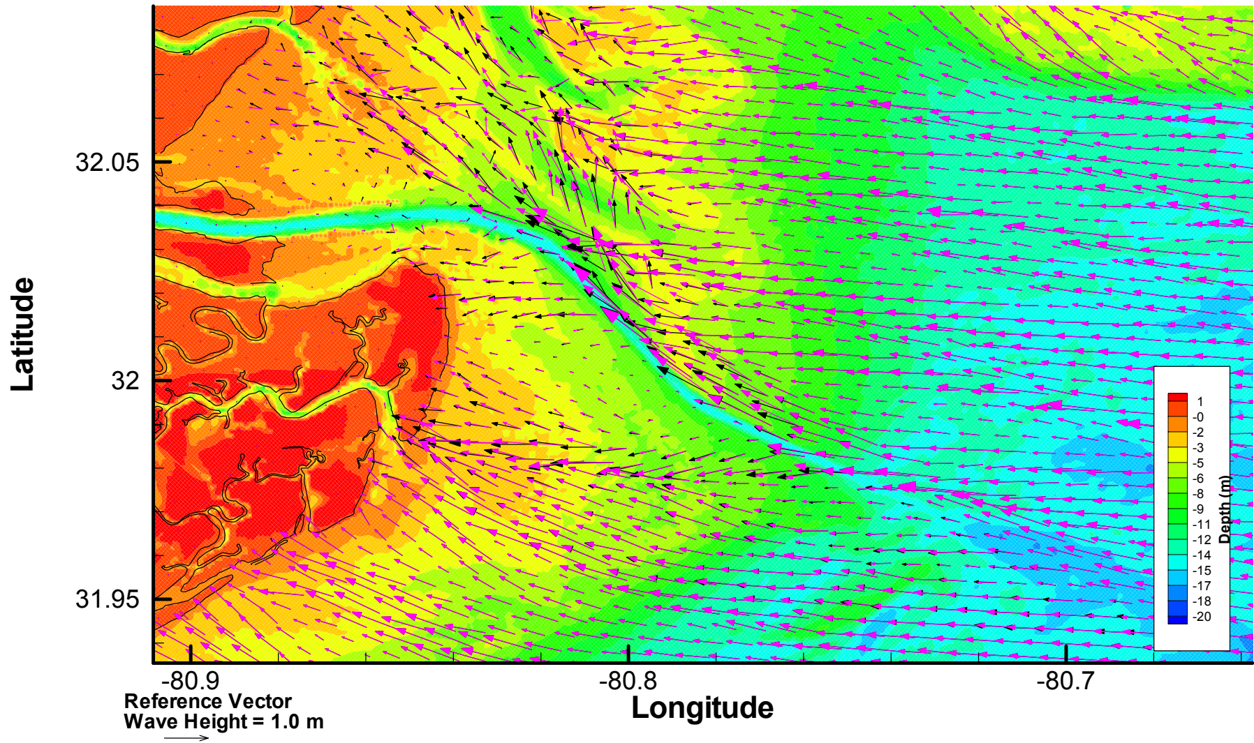
Figure A-1 Simulated pre- and post-project Case 1 average wave conditions over the entire model grid. (black vectors=pre-project, purple vectors=post-project)
